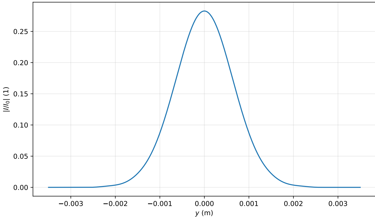
Intensity profile I(x=0, y, z=3.662)/I_0 , P_{in}=0.2P_{cr} , artificial time
